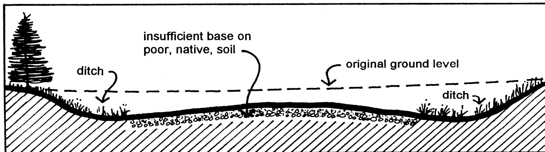
Figure 5. Poorly constructed road: poor base, inadequate ditching and built below original ground level.
